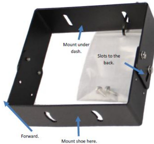
Figure A.3: Under-Dash Mount - Kit.
